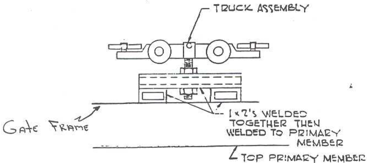
DETAIL C ATTACHMENT OF TRUCK ASSEMBLY TO GATE
