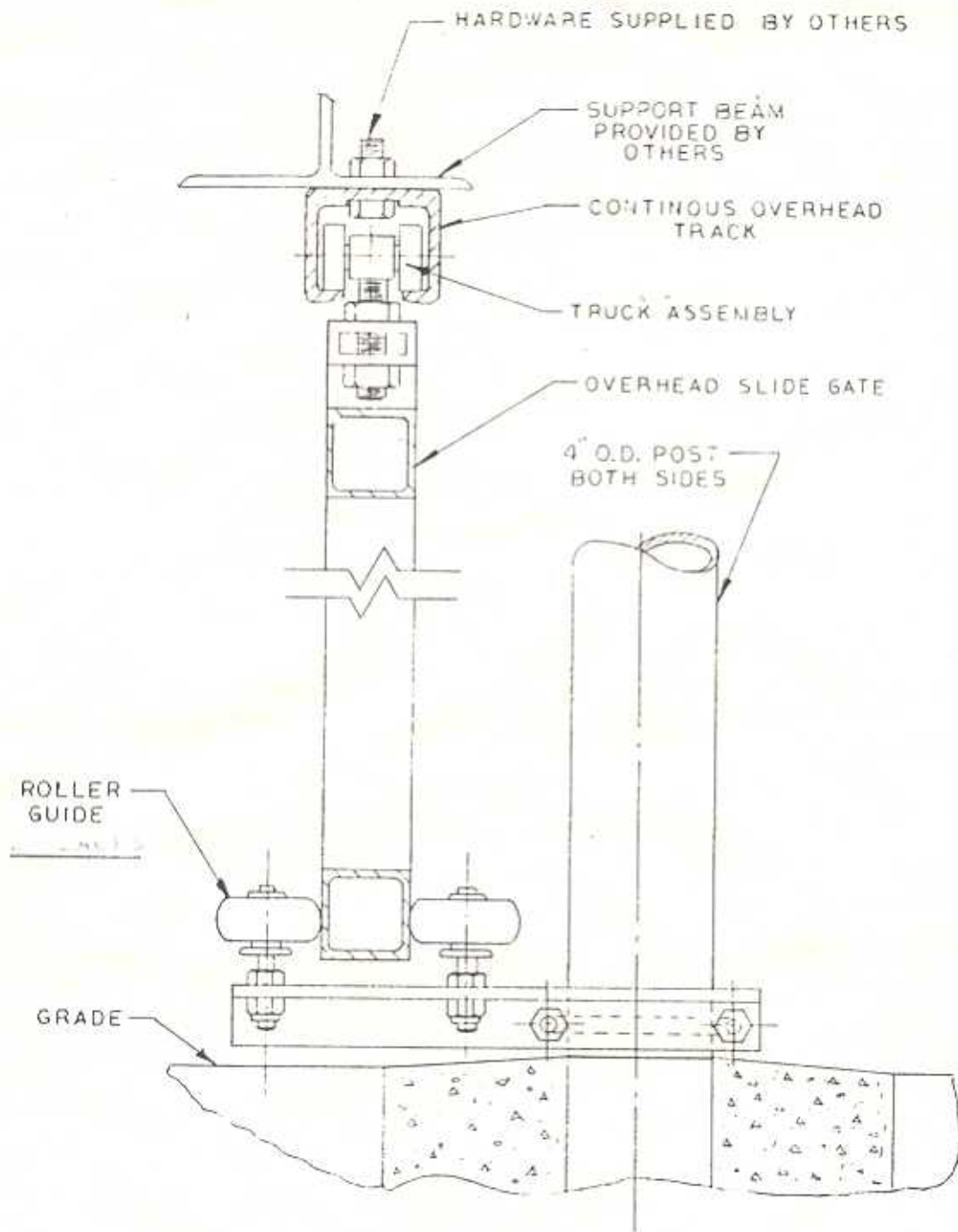
SECTION B-B (TYPICAL FREE STANDING INSTALLATION)
